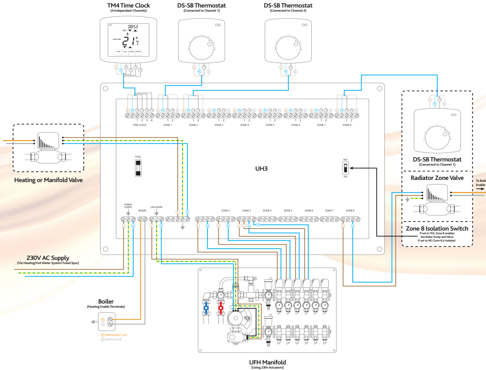
8 Zone Wiring Centre Part Ref: Heatmiser UH3
